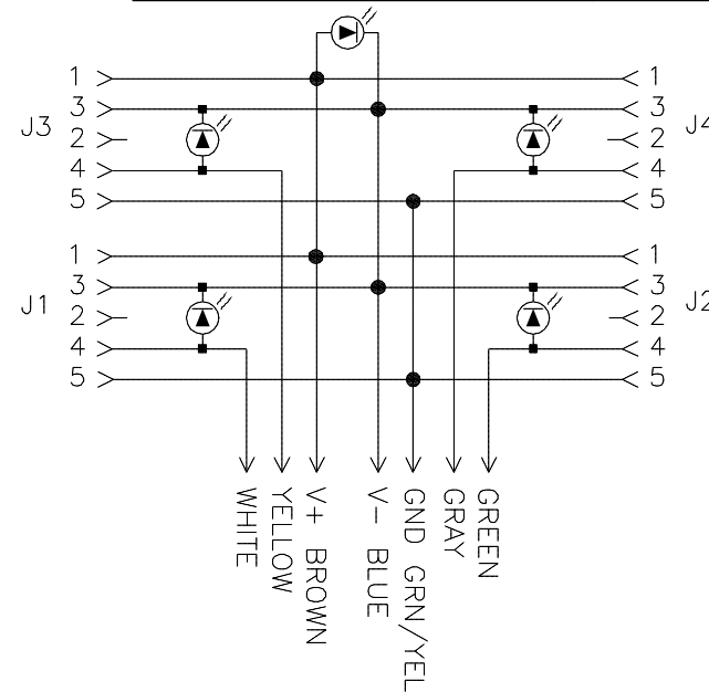
WIRING DIAGRAM
